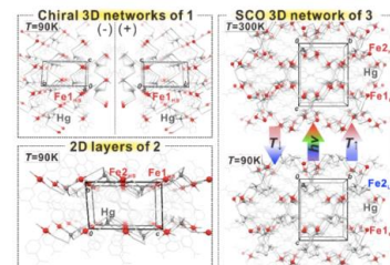
Fig 1. Structures of 1 - 3
