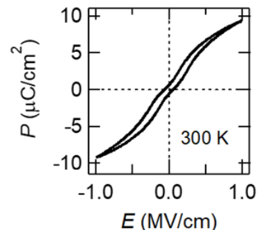
Figure 1. P - E (a) curve of the h\text{-DFO} film measured at 300 K and 5 kHz
