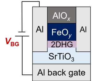
Fig. 1: Schematic cross-sectional structure of the \text{AlO}_x/\text{FeO}_y/\text{STO} samples with Al back gate and contact pads.
