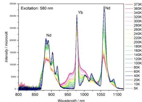
Figure 1. T-dependence of NIR-photoluminescent emission spectra after dehydration ( x=0.71 , y=0.29 ).
