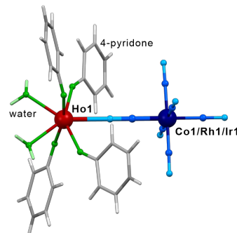
Fig 1. Structure of 1-3
