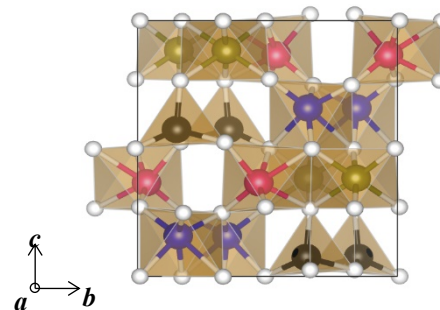
Figure1: The crystal structure of \epsilon - Fe 2 O 3
