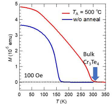
Fig. 1. Increase of T_C by post-growth annealing in \text{Cr}_3\text{Te}_4 .
